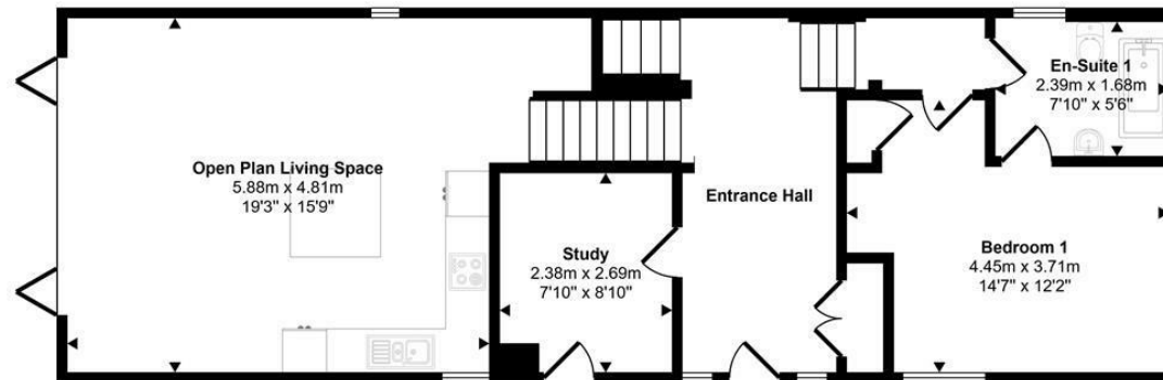
Ground Floor Approx 74 sq m / 799 sq ft
